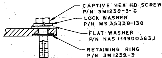
DETAIL A 4 PLACES ROTATED 90° SCALE 2:1
