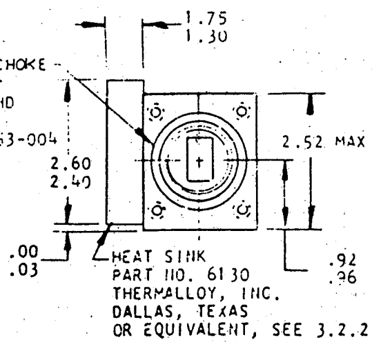
FIGURE 1. OUTLINE DRAWING
