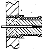
TYPICAL BLIND MATE RS PART NO 24011-3-1 DETAIL VIEW
